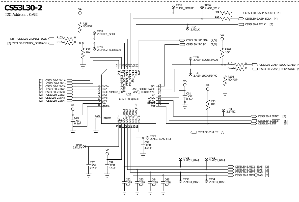
Figure 6-1. CS53L30
